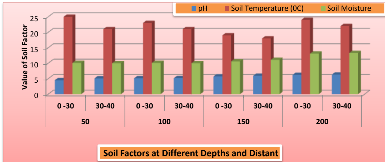
Fig.1: Variation of Soil Factors at different Depths and Distant
