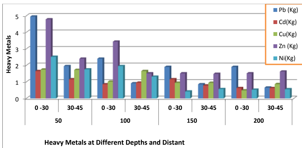
Fig.2: Variation of Heavy Metal Concentrations in the Soil at Graded Distance
