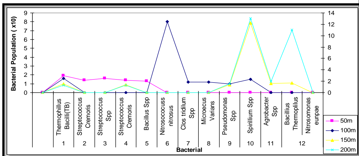
Fig.3: Variations of Bacterial Population in the Soil with Distance from the Roadside
